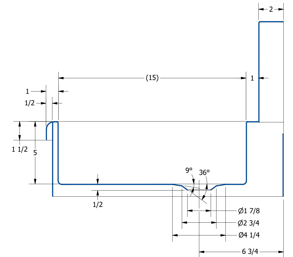
SECTION A-A SCALE 1 / 4
